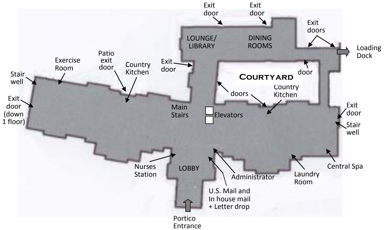
FIRST FLOOR
